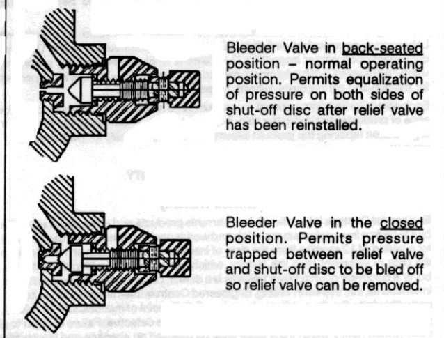
Figure 2: Bleeder Valve Detail
