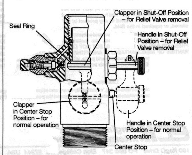
Figure 3: Side view without relief valves
